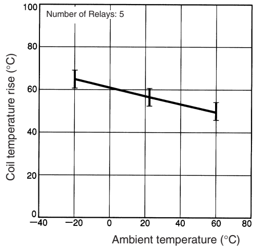
G7J-4A 24 VDC
